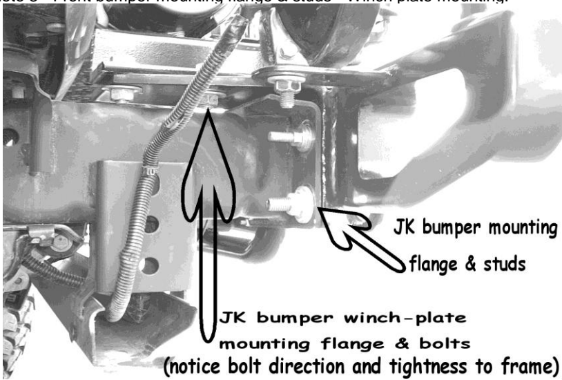
Photo 3 - Front bumper mounting flange & studs - Winch plate mounting.
